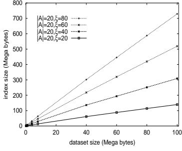
(a) Uniform symbol dist., |A| = 20
