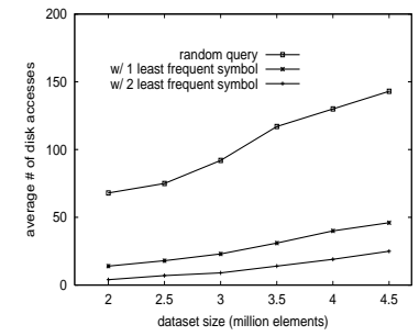
(b) Subsequence Reordering
