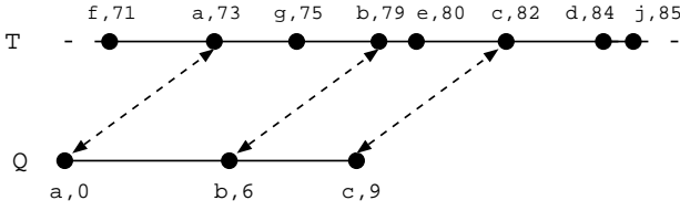
Figure 2. Query Q = \langle (a, 0), (b, 6), (c, 9) \rangle matches a non-contiguous subsequence of T, \langle (a, 73), (b, 79), (c, 82) \rangle
