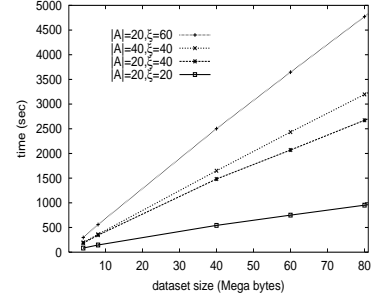
(a) Uniform symbol dist.
