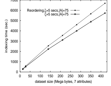
(b) TEC: 75 symbols (Zipf-like dist.)
