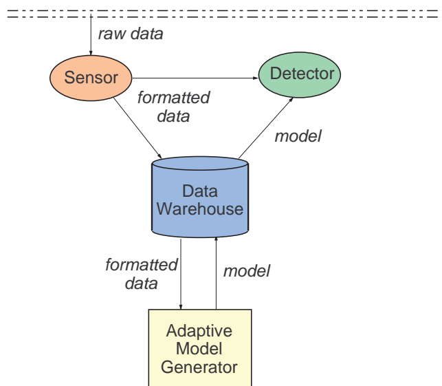
Figure 2. The Architecture of Data Mining-based IDS
